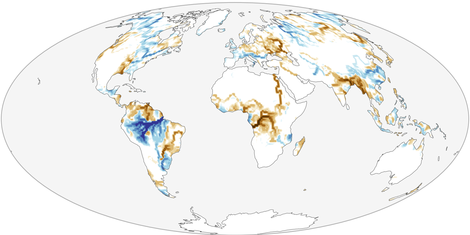
Difference from average river runoff (meters 3 per second)
